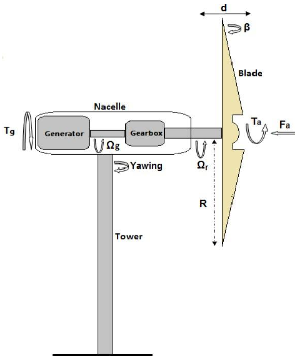
Figure 1.1 Wind turbine with horizontal Axis.
