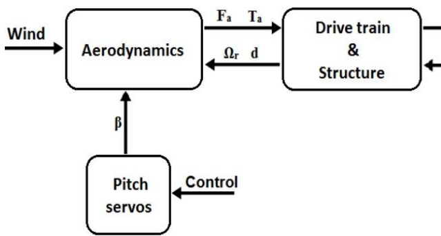
Figure 1.2 Sub System-level block diagram of a variable speed variable – pitch (VS-VP) Wind Turbine.
