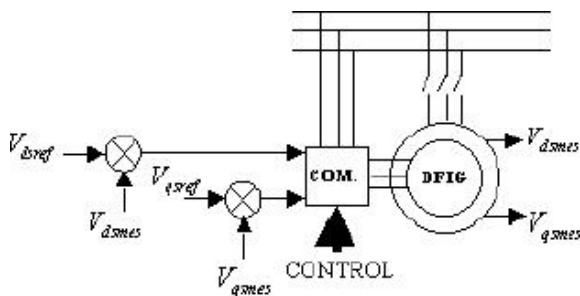
Figure 2.2 DFIG Control Step 1.
