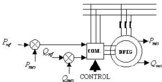
Figure 2.3 DFIG control Step 3.
