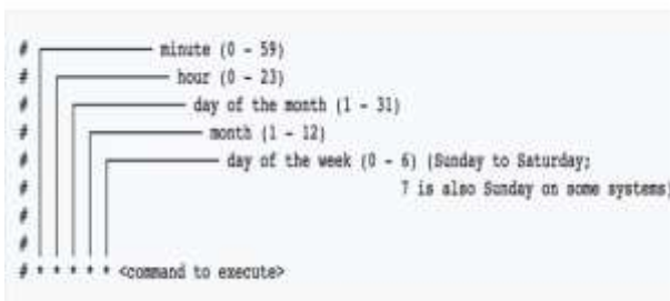
Fig. 2. Nature of cron syntax
