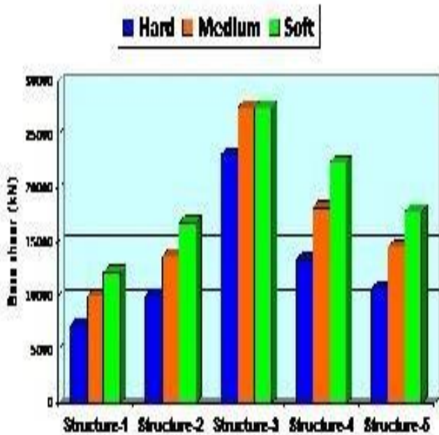
Figure 6.2: variations in base shear for all structure with load combination
