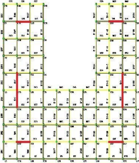
Fig.-2.Plan of structures 2 at Basement level
