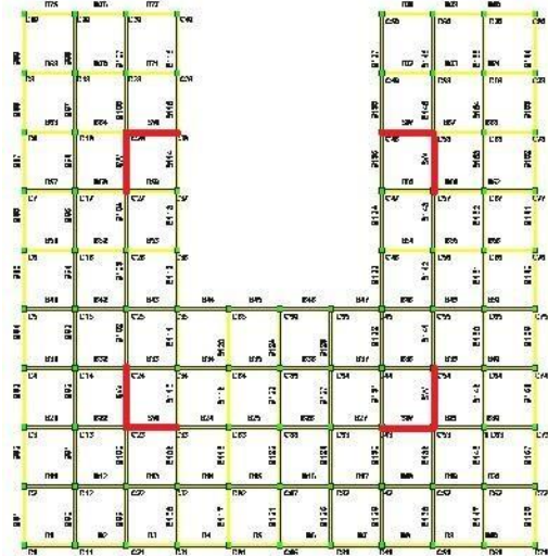
Fig.-5.Plan of structures 5 at Basement level
