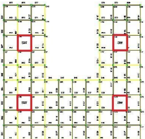
Fig.-4.Plan of structures 4 at Basement level
