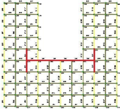
Fig.-3.Plan of structures 3 at Basement level
