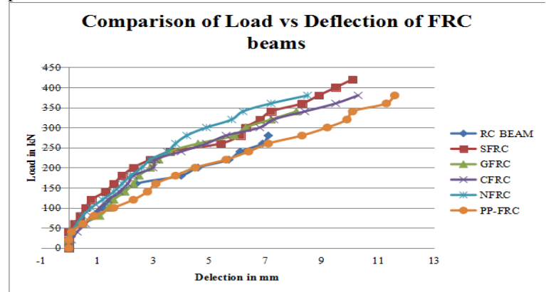
Load Vs. Deflection curve comparison for all beam specimens
